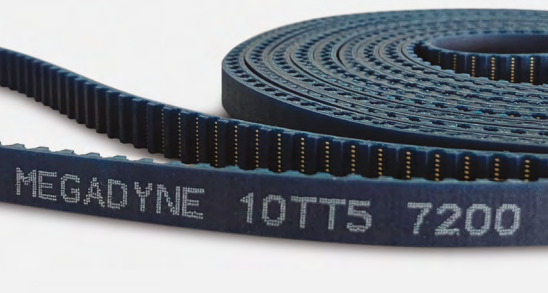
TOOTH PROFILE ACCORDING DIN 7721-1
