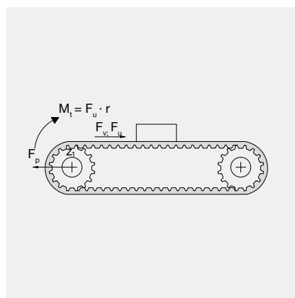
Conveyor transmission
