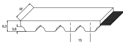
TOOTH PROFILE ACCORDING ISO 17396
